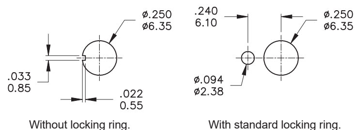
PANEL MOUNTING
